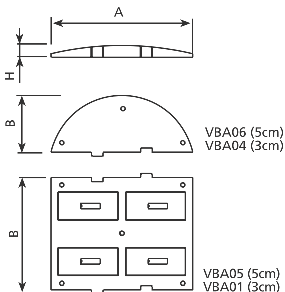
152. PARKING STUPIČI
